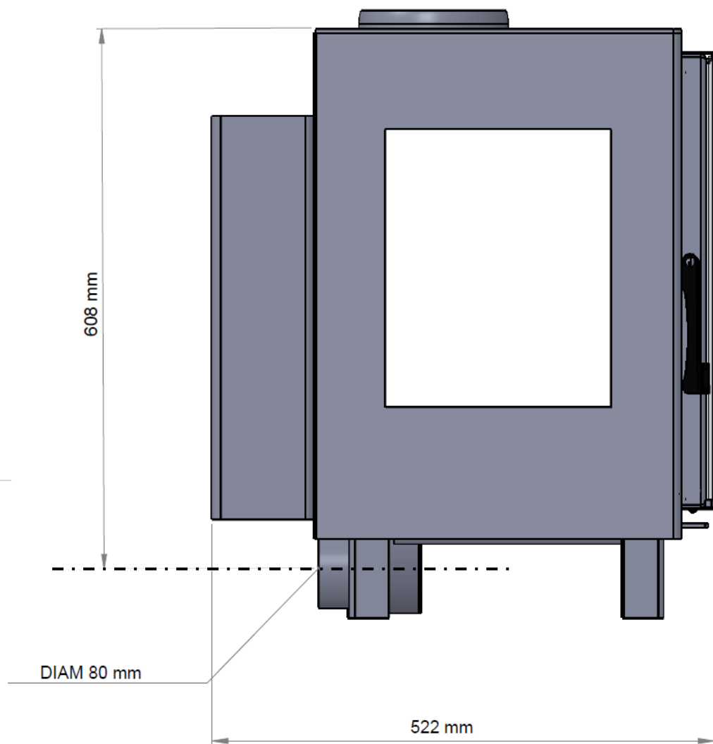
Illustration1. General plan
