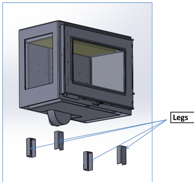
Illustration11. Position of the legs and their screws
